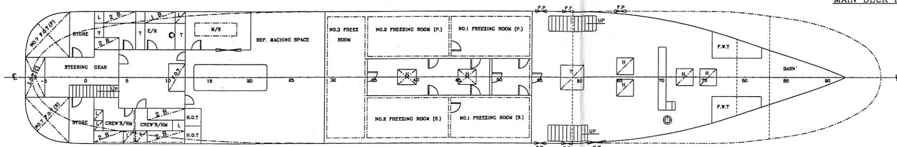
MAIN DECK PLAN
