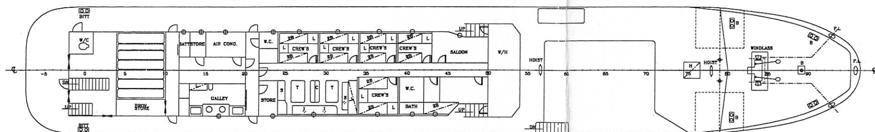
MAIN DECK PLAN
